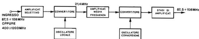
Fig. 3.29 Transposer FM
